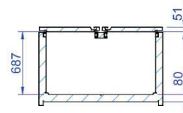
SECTION C-C
