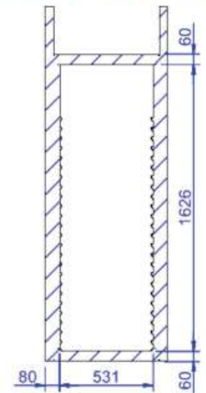
SECTION B-B
